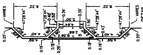
DETAIL TYPICAL DECK AND ADJACENT BAY WINDOW UNITS ON 3RD - 5TH FLOOR (NOT TO SCALE)
