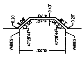
DETAIL TYPICAL BAY WINDOW UNITS ON 3RD - 5TH FLOOR (NOT TO SCALE)
